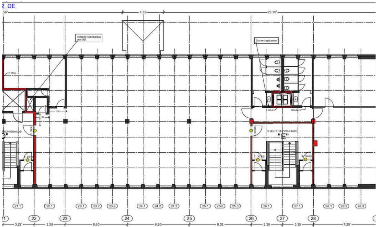
Grundriss | Plan
