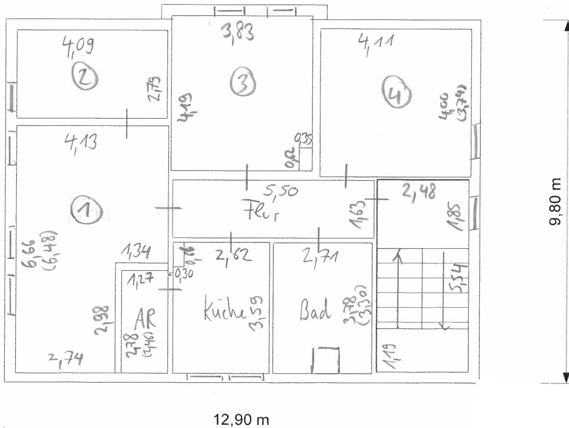
Grundriss DG, M = 1:100
