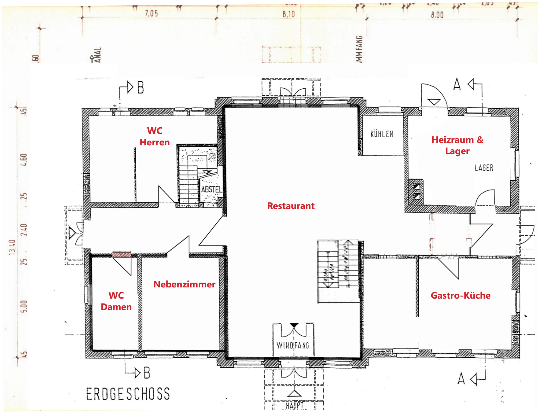
Grundriss Erdgeschoss RESTAURANT
