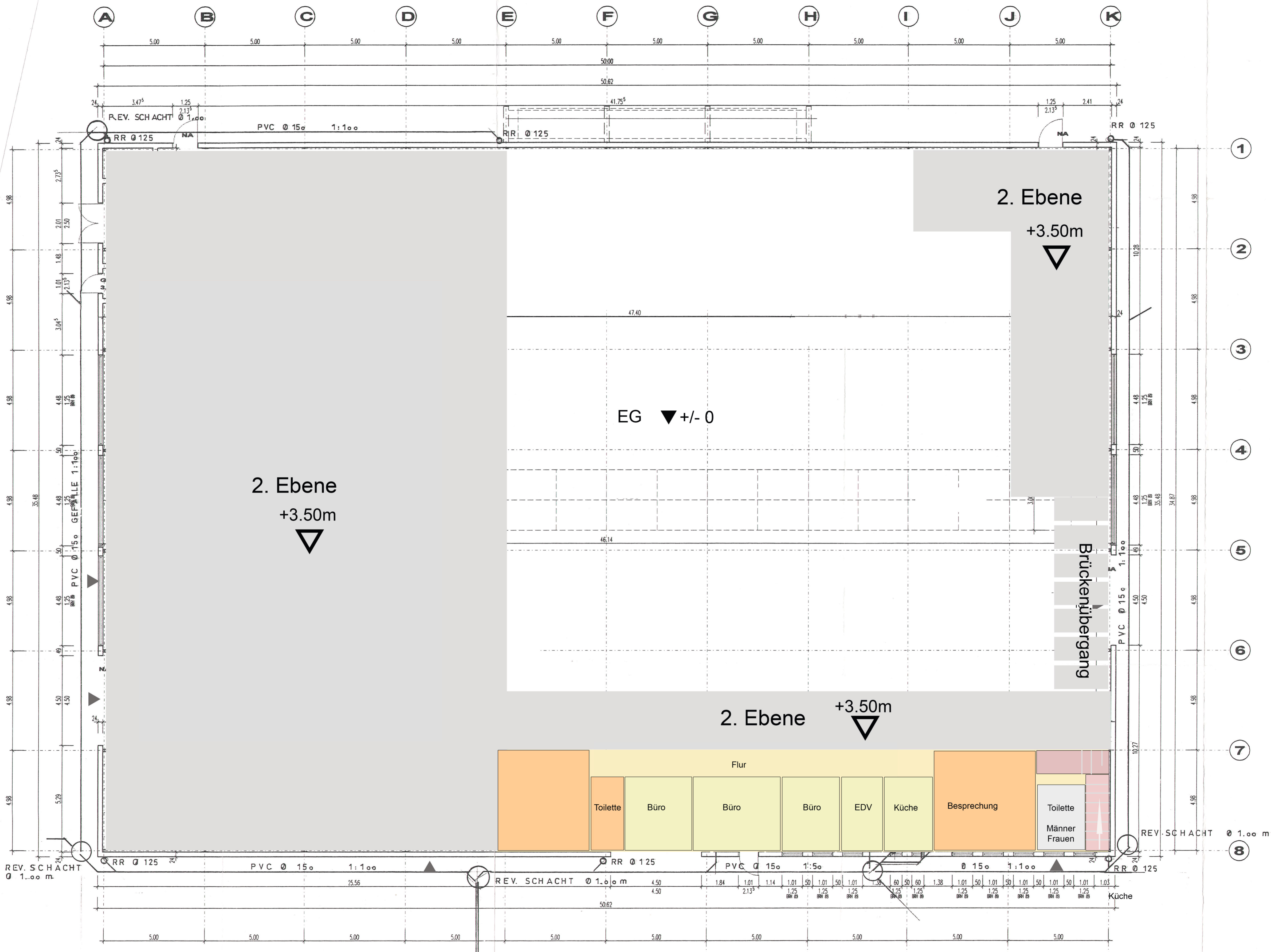
Grundriß - Erdgeschoß
