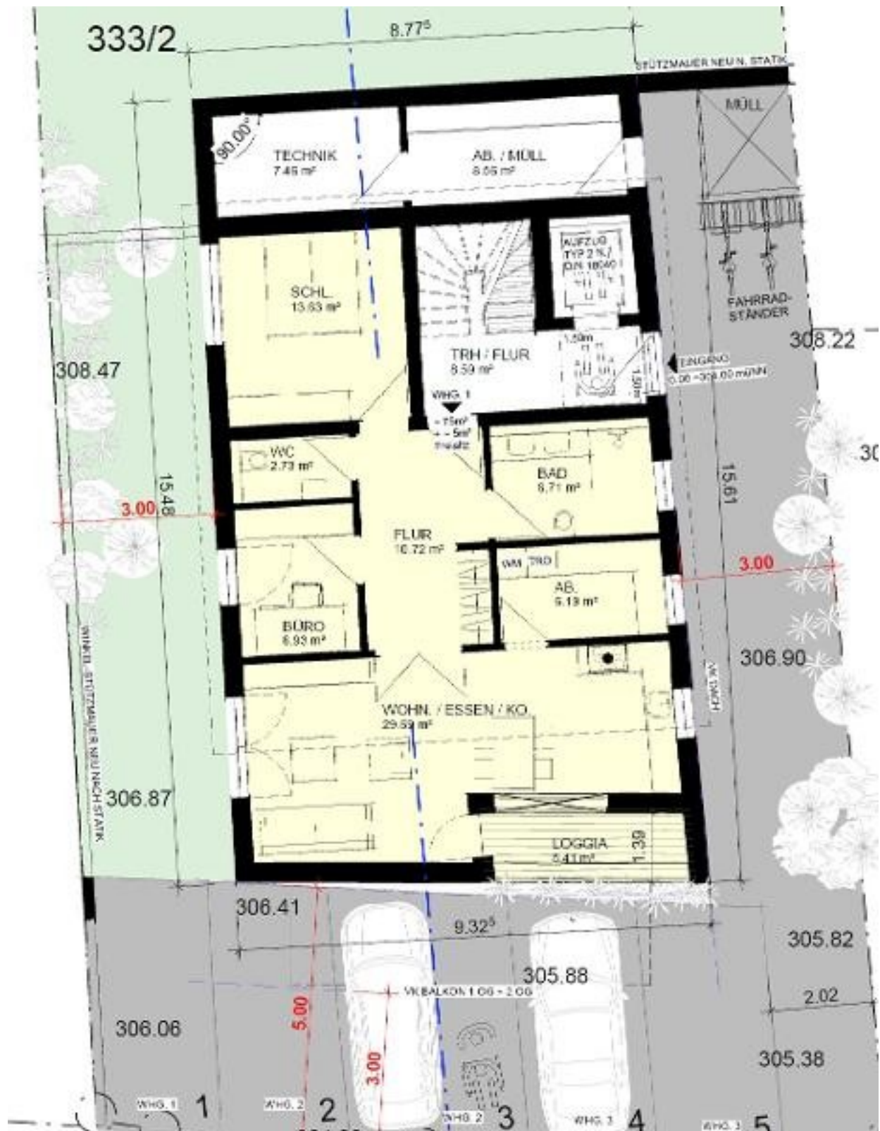
Grundriss WHG 1
